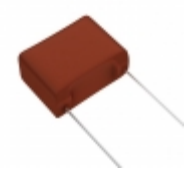
ECW-F2275JA Panasonic Electronic Components CAP FILM 2.7UF 5% 250VDC RADIAL
