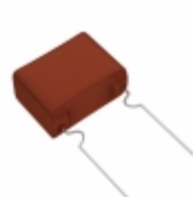
ECW-F2275HAB Panasonic Electronic Components CAP FILM 2.7UF 3% 250VDC RADIAL
