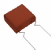
ECW-F2275HAQ Panasonic Electronic Components CAP FILM 2.7UF 3% 250VDC RADIAL
