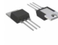
L4006L8 Littelfuse Inc. TRIAC SENS GATE 400V 6A TO220
