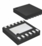
MIC5314-F4YMT-TR Microchip Technology IC REG LDO 1.5V/1.2V 0.3A 12TMLF
