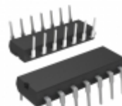
MCP42050-I/P Microchip Technology IC POT DGTL 50K 2CH SPI 14-DIP
