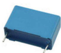
B32523Q3155K EPCOS (TDK) CAP FILM 1.5UF 10% 250VDC RADIAL
