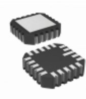
AD827SE/883B Analog Devices Inc. IC OPAMP GP 50MHZ DUAL LP 20CLCC
