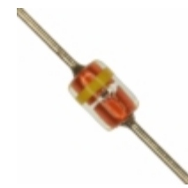
MTZJT-727.5A Rohm Semiconductor DIODE ZENER 7.5V 500MW DO34
