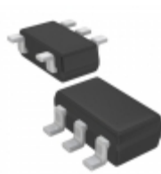
MCP40D19T-503E/LT Microchip Technology IC DGTL POT 50K 128TAPS SC70-5
