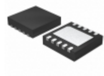
MIC61300-10YML-TR Microchip Technology IC REG LDO 1V 3A 10MLF
