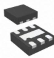
MIC94345-MYMT-T5 Microchip Technology IC REG LDO 2.8V 0.5A 6TDFN
