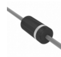
P6KE56A-E3/54 Electro-Films (EFI) / Vishay TVS DIODE 47.8V 77V DO204AC
