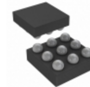
ADA4691-2ACBZ-R7 ADI (Analog Devices, Inc.) IC OPAMP VFB 3.6MHZ RRO 9WLCSP
