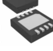
ADA4666-2ACPZ-RL ADI (Analog Devices, Inc.) IC OPAMP GP 4MHZ RRO 8LFCSP
