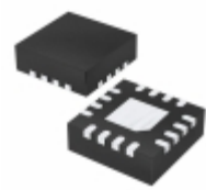
MCP4641T-104E/ML Microchip Technology IC DGTL POT 100K 129TAPS 16-QFN
