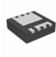
BSZ084N08NS5ATMA1 Infineon Technologies MOSFET N-CH 80V 40A 8TSDSON
