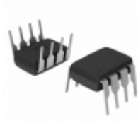
AT24C16-10PC-2.7 Microchip Technology IC EEPROM 16KBIT 400KHZ 8DIP
