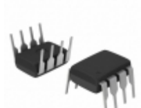
TC426CPA Microchip Technology IC MOSFET DVR 1.5A DUAL HS 8- DIP
