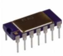
AD536AJD Analog Devices Inc. IC TRUE RMS/DC CONV 14-CDIP
