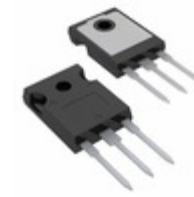
IRG4PC60U-PPBF Infineon Technologies IGBT 600V 75A 520W TO247AC
