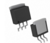
MIC2940A-3.3WU-TR Microchip Technology IC REG LDO 3.3V 1.25A TO263-3
