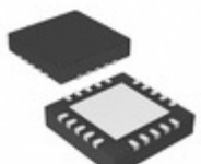
MCP4451T-503E/ML Microchip Technology IC DGTL POT 257POS 50K 20QFN
