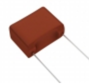
ECW-FA2J155J Panasonic Electronic Components CAP FILM 1.5UF 5% 630VDC RADIAL
