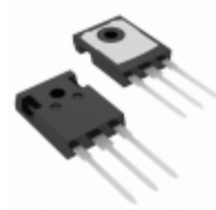
FGH30N6S2D Fairchild/ON Semiconductor IGBT 600V 45A 167W TO247
