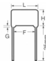
ECQ-P1H471JZ3 Panasonic Electronic Components CAP FILM 470PF 5% 50VDC RADIAL
