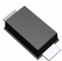
KDZTR7.5B Rohm Semiconductor DIODE ZENER 7.9V 1W PMDU
