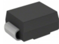
CEFB102-G Comchip Technology DIODE GEN PURP 100V 1A DO214AA
