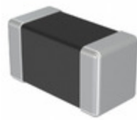
TMK042CG2R9BD-W Taiyo Yuden CAP CER 2.9PF 25V COG/NP0 01005
