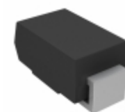
SML4762HE3/5A Vishay Semiconductor Diodes Division DIODE ZENER 82V 1W DO214AC
