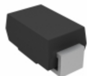
SML4762HE3/61 Vishay Semiconductor Diodes Division DIODE ZENER 82V 1W DO214AC
