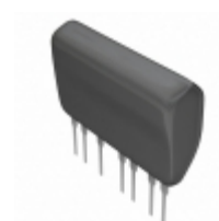
BP5710-1 Rohm Semiconductor AC/DC CONVERTER 12V 350MA 4W
