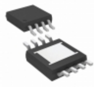
LT3061EMS8E-5#PBF ADI (Analog Devices, Inc.) IC REG LINEAR 5V 100MA 8MSOP
