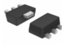
MC78LC50HT1 ON Semiconductor IC REG LDO 5V 80MA SOT89-3
