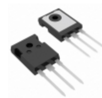
IXGH100N30C3 IXYS IGBT 300V 75A 460W TO247
