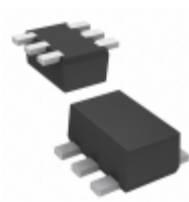
UP0453400L Panasonic Electronic Components TRANS 2NPN 20V 0.015A SSMINI6
