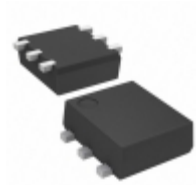
MTM861270LBF Panasonic Electronic Components MOSFET P-CH 20V 2A WSSMINI6
