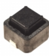
KSH451J 50 LFS C&K SWITCH TACTILE SPST-NO 50MA 12V
