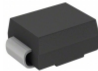
SMBJ58A Littelfuse Inc. TVS DIODE 58VWM 93.6VC SMB
