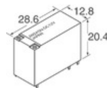
JW2SN-DC60V Panasonic Electric Works JW RELAY 2 FORM C 60V 5A
