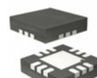
AD8465WBPCZ-WP Analog Devices Inc. IC COMPARATOR 1CH LVDS 12LFCSP
