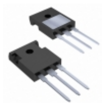
IXTJ4N150 IXYS MOSFET N-CH 1500V 2.5A ISOTO-247
