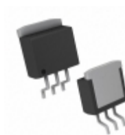
MCP1827ST-3302E/EB Microchip Technology IC REG LDO 3.3V 1.5A 3DDPAK
