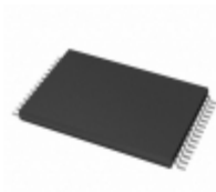
AT28HC64B-70TI Microchip Technology IC EEPROM 64KBIT 70NS 28TSOP
