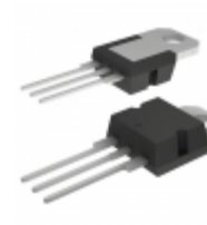
MIC2940A-5.0BT Microchip Technology IC REG LDO 5V 1.25A TO220-3
