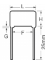
ECQ-P1H472GZ3 Panasonic Electronic Components CAP FILM 4700PF 2% 50VDC RADIAL
