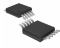
LTC2433-1IMS#TRPBF Linear Technology IC ADC DIFF 16BIT 3WIRE 10-MSOP
