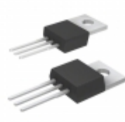
IXFP7N80PM IXYS MOSFET N-CH 800V 3.5A TO-220
