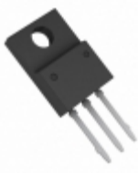
BA7806CP-E2 Rohm Semiconductor IC REG LDO 6V 1A TO220CP-3
