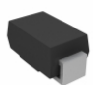
P4SMA18A-E3/61 Vishay Semiconductor Diodes Division TVS DIODE 15.3VWM 25.2VC SMA
