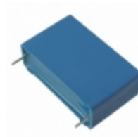
B32676G3206K EPCOS (TDK) CAP FILM 20UF 10% 300VDC RADIAL
