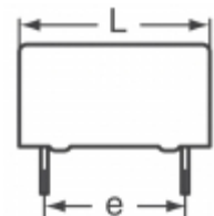
B32676G3256K EPCOS (TDK) CAP FILM 25UF 10% 300VDC RADIAL
