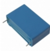
B32676G1905J000 EPCOS CAP FILM 9UF 5% 750VDC RADIAL
