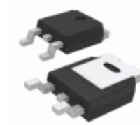
STD5NK52ZD STMicroelectronics MOSFET N-CH 520V 4.4A DPAK
