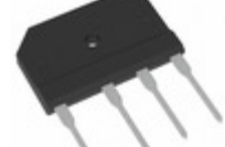
TS35P06GHD2G TSC (Taiwan Semiconductor) BRIDGE RECT 1P 800V 35A TS-6P
