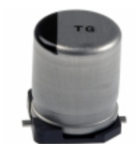
EEV-TG1H470UP Panasonic Electronic Components CAP ALUM 47UF 20% 50V SMD
